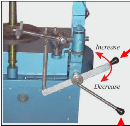
Lever for Adjusting carving Pressure
